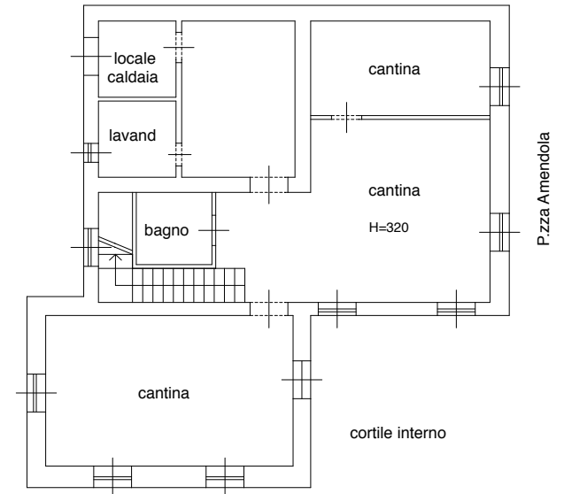
PIANO CANTINATO
