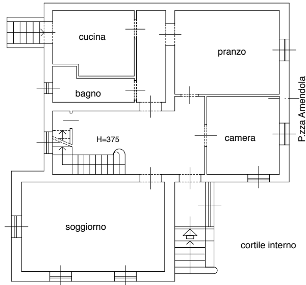
PIANO TERRENO
